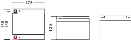
Terminal Dimensions
